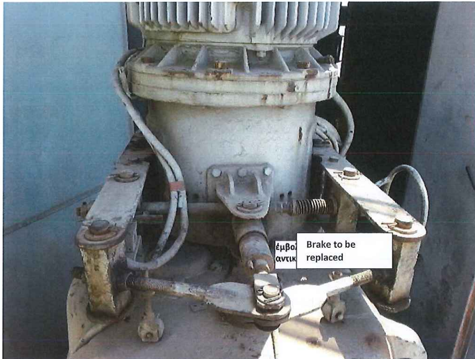
1st photo: Configuration of brake to be replaced E/C 31 same as E/C 32.
